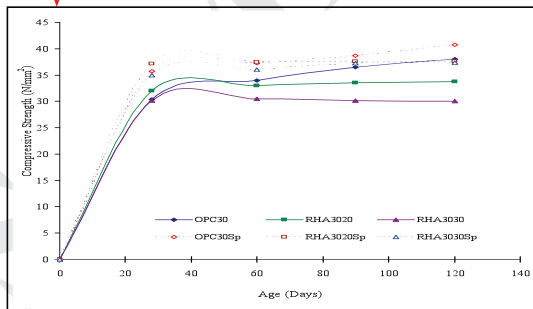
Figure 4.1 Compressive Strength of Rice Husk Ash (RHA) Concrete of Grade 30
